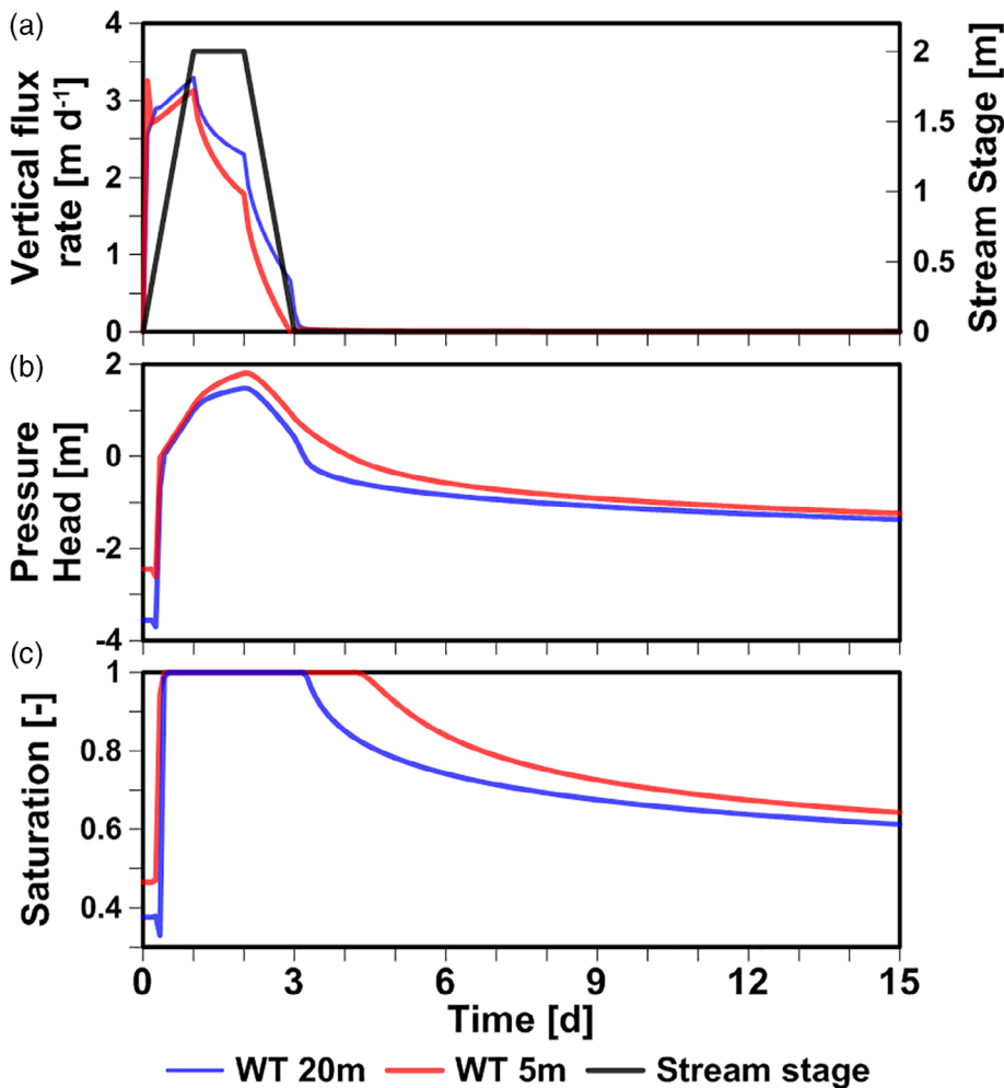
FIGURE 4 Temporal variation modelled at 1 m below the centre of stream (left side of model half-space) for the same scenarios of Figure 3: (a) infiltration rate, with stream stage shown for comparison on right-hand axis, (b) pressure head and (c) degree of saturation for deeper (20 m) and shallower (5 m) water tables (WT). Soil parameters correspond to the base case scenario (Figure 2)
