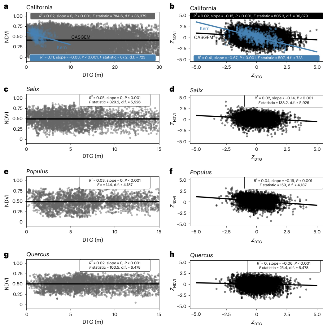
Fig. 4 | NDVI vs DTG plots and Z_{NDVI} vs Z_{DTG} plots for groundwater-dependent vegetation across California. a–h NDVI vs DTG plots (left) and Z_{DTG} vs Z_{NDVI} plots (right) for groundwater-dependent vegetation across California (a, b; n = 3,113 polygons with statewide CASGEM monitoring well data in grey/
