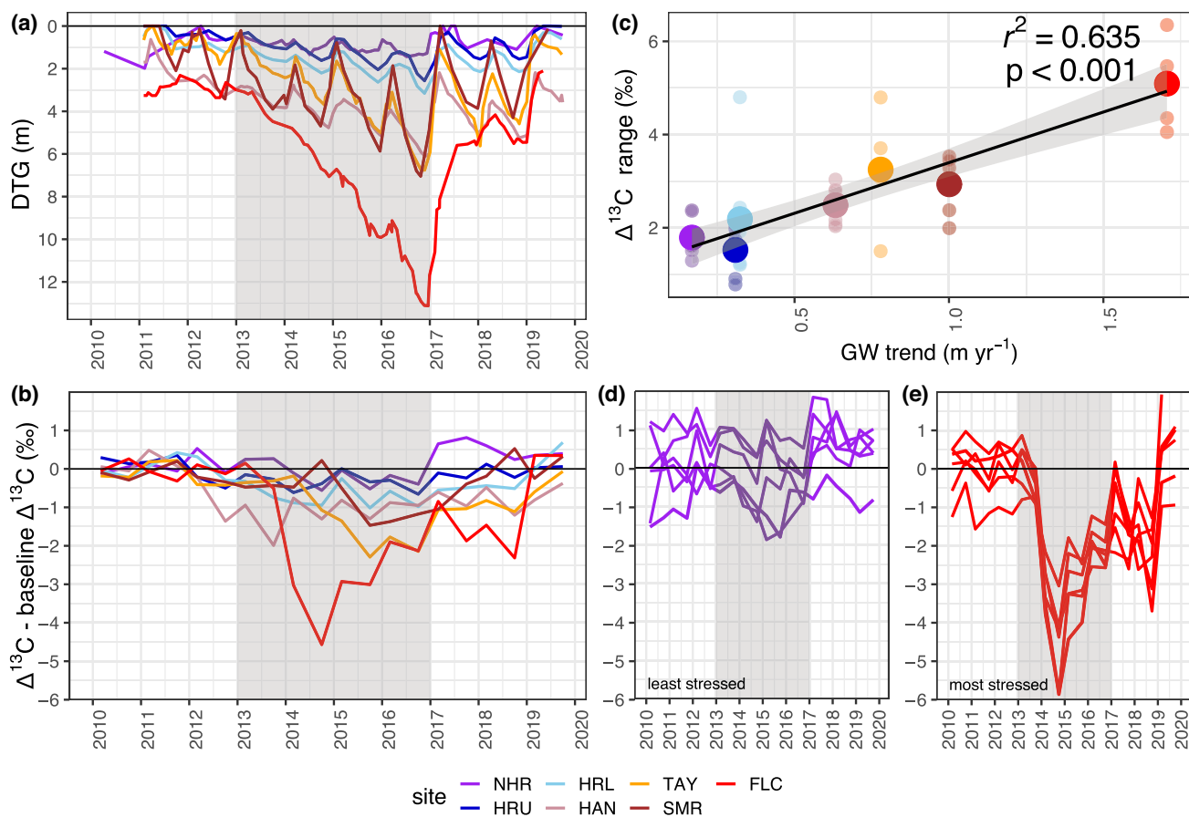
FIGURE 4 (a) All depth to groundwater (DTG) observations for each site along the lower Santa Clara River, California. The horizontal line represents the land surface, and the vertical axis is inverted to depict increasing DTG. (b) Complete time series of site mean \Delta^{13}\text{C} residuals for earlywood and latewood combined as seasonal series (i.e., two values per year) for each site. The horizontal line depicts baseline \Delta^{13}\text{C} . (c) Scatterplot of \Delta^{13}\text{C} range (max \Delta^{13}\text{C} - Min \Delta^{13}\text{C} ) values from 2010 to 2019 for each tree (small points) and the average of these values for each site (large points). The horizontal axis is the interannual groundwater trend calculated for each site by applying Sen's slope to median annual DTG values from 2011 to 2016. The trendline was calculated with values from all trees (small points) and displayed with standard error of the slope (shaded area) along with r -squared value and significance value of slope. (d) Complete time series of \Delta^{13}\text{C} residuals for individual trees at Newhall ranch, the site with the shallowest groundwater decline. (e) Same as previous panel but for Fillmore Cienega, the site with the steepest groundwater decline. Grey shading in plots denotes the peak hydrological drought period (2013–2016).
